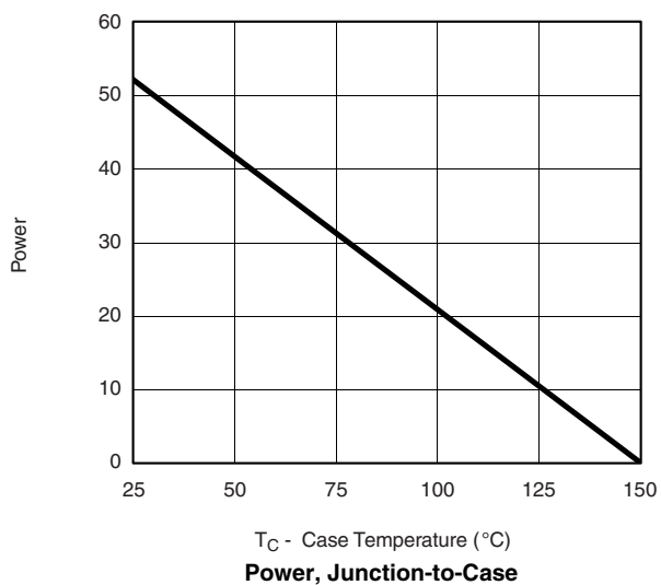
Power, Junction-to-Case
