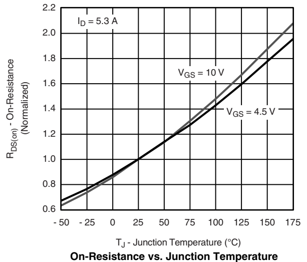
I_D = 5.3\text{ A} V_{GS} = 10\text{ V} V_{GS} = 4.5\text{ V} On-Resistance vs. Junction Temperature
