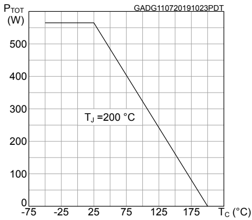
Figure 9. Maximum total power dissipation
