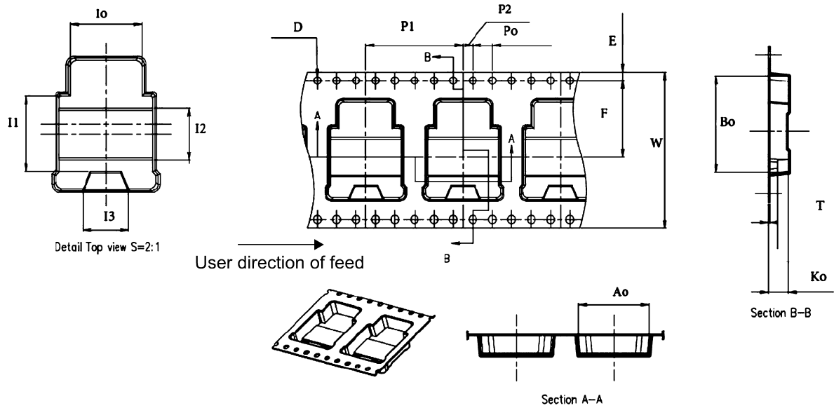
Figure 19. HU3PAK carrier tape outline
