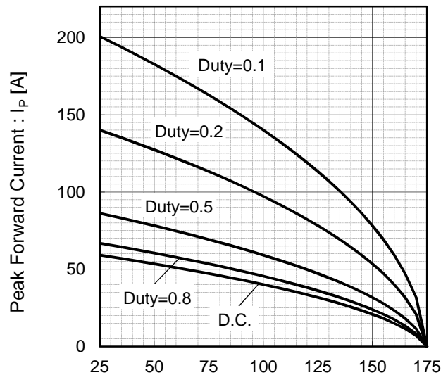
Fig.8*4 Typical peak forward current derating curve I_P - T_c (Not guaranteed)
