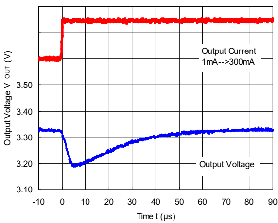
RP550K001A ( V_{IN}=5.0V , V_{OUT}=3.3V ) MODE="H" Forced PWM Control
