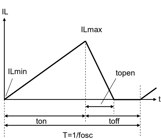
Figure 5. Discontinuous Mode
