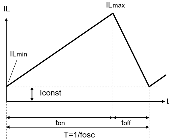
Figure 6. Continuous Mode
