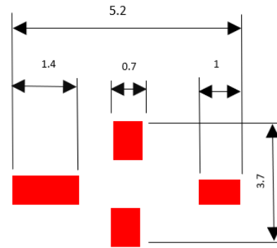
PCB Footprint
