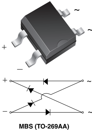
MBS (TO-269AA)
