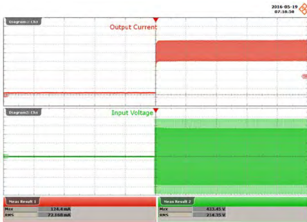
Figure 63 – 30 VAC, 48 V LED, Output Rise. Upper: I_{OUT} , 40 mA / div. Lower: V_{IN} , 100 V / div., 1 s / div.
