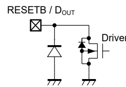
Equivalent Circuit for RESETB Pin (R5115Sxx1x)/ Equivalent Circuit for DOUT Pin (R5115xxx2C)
