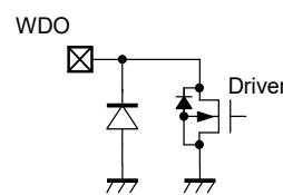
Equivalent Circuit for WDO Pin (R5115xxx2C)
