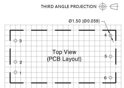
Note: Grid 2.54*2.54mm
