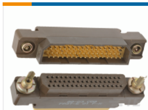
TE Part #ZPF00000000017894 FAST-E 07 M-X-A 00 A
