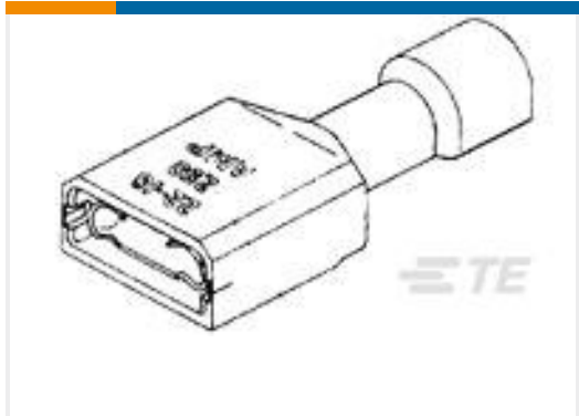
TE Part #3-520140-4 ULTRA-FAST 250 ASY REC 16-14 AWG TPBR
