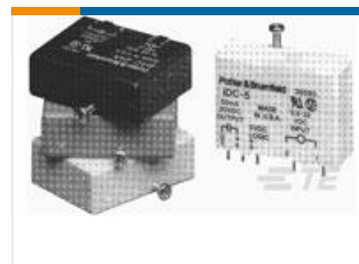
TE Part #6-1393028-9 OAC-5 = PCB mount, 3A, 120V AC - DC I/p
