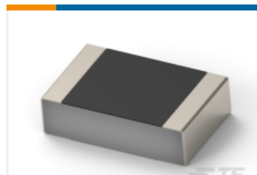
TE Part #8-2176453-5 CPF 0201 43K2 0.1% 25ppm 1K RL
