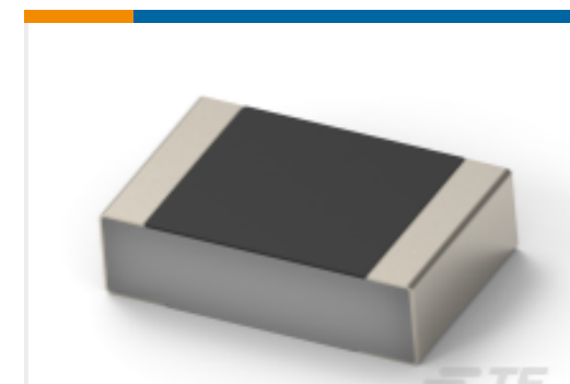
TE Part #8-2176453-6 CPF 0201 44K2 0.1% 25ppm 1K RL
