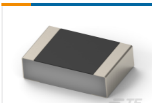
TE Part #8-2176453-2 CPF 0201 40K2 0.1% 25ppm 1K RL
