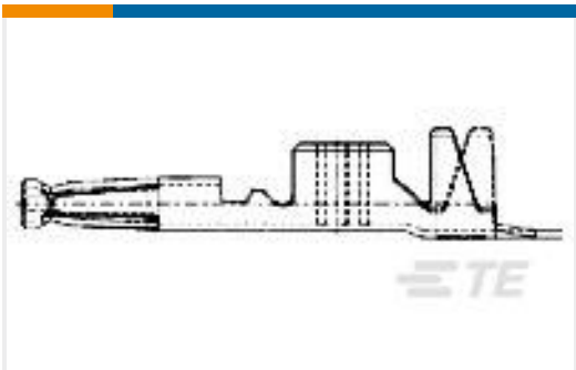
TE Part #1719532-1 MQS0,63 Sn rec CB unseal. AWG18
