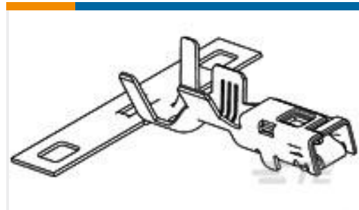
TE Part #1326032-4 2.8MM RECP,SEAL,16AWG
