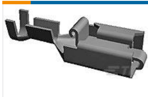
TE Part #341002-6 PL 250 REC TERMINAL 18-14 PTPB LP
