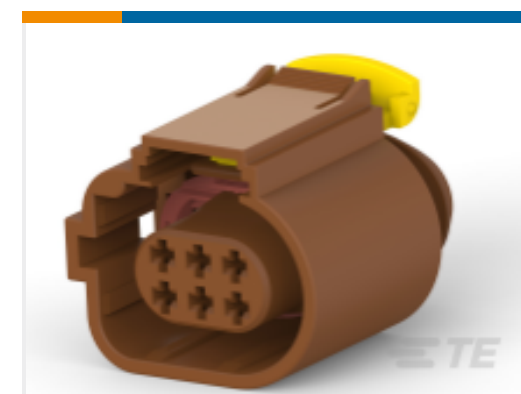
TE Part # 1-284716-3 6 POS REC. CONNECTOR FOR MTII
