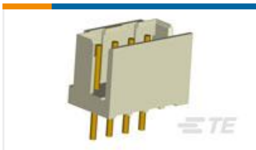
TE Part #292132-7 CT P/HDR BOX V 7P NAT
