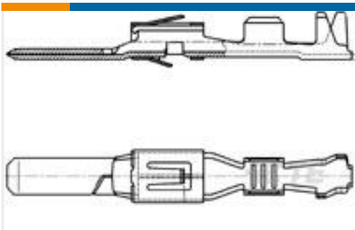
TE Part #962884-1 TAB AS 2.8x0.8 CONTACT CS SRC Sn
