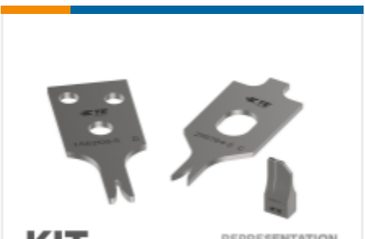
TE Part #7-2266792-7 OCEAN_2.0_SPARE_PART_KIT- 108F138F
