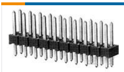
TE Part #1-829315-0 2X10P MOD2 STIFTELEI
