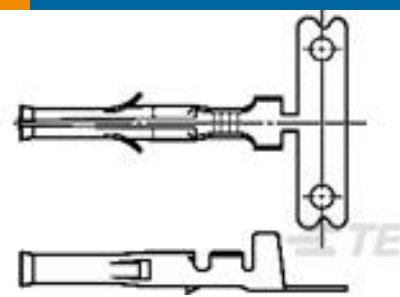
TE Part #794046-1 .062 COMM P&S SOK 24-30 PTPBR
