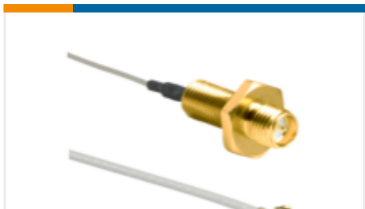
TE Part #CSI-RGFE-300-UFFR RP-SMA to U.FL/MHF1 300mm 1.13 OD
