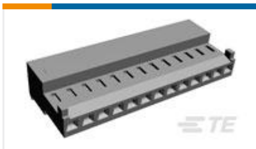
TE Part #4-644083-3 13P MTA100 CONN ASSY POL TAB
