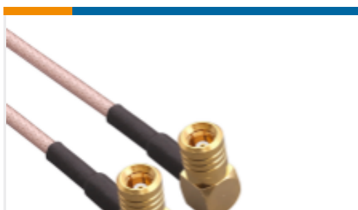
TE Part #CSE-SBRM-152-SBRM SMB to SMB 152mm RG316
