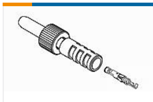
TE Part #5-861610-2 LGH, HIGH VOLTAGE PLUG
