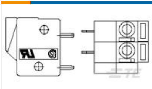
TE Part #1776261-2 Bd Mt Screwless, 5.0mm, Side W
