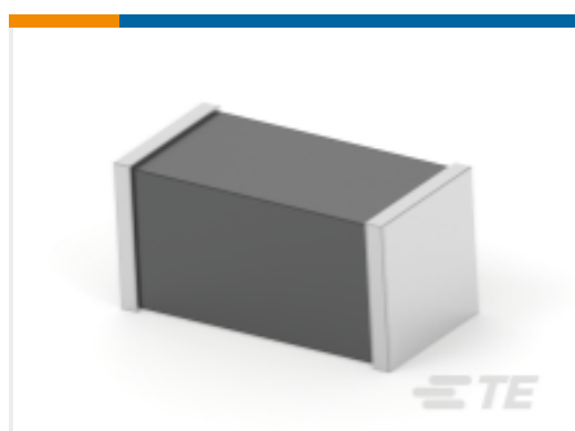
TE Part #2176493-8 BMC 0603 120R 25% A Gen C
