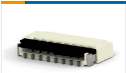
TE Part #2-2328724-1 21PIN 0.3MMP FPC CONNECTOR, FRONT FLIP
