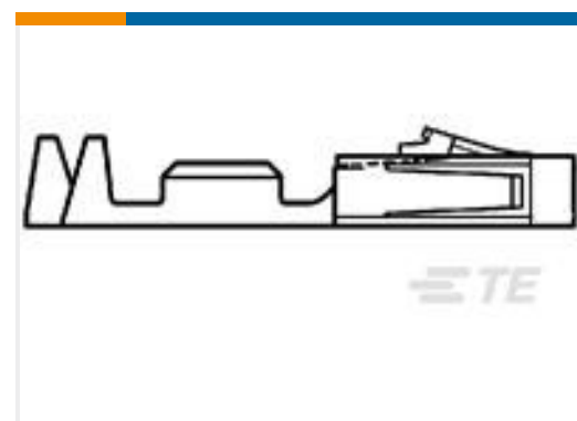
TE Part #1-104480-4 SHORT POINT RECP CONT LP
