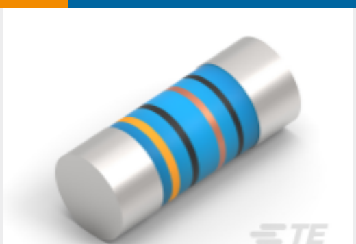
TE Part #2176314-1 MELF SMA_A 100R 0.1% 15PPM 0102 0.3W
