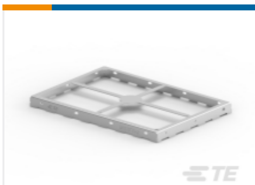
TE Part #2118730-2 STD SHIELD FRAME, CRS-44.00X30. 50X3.00MM
