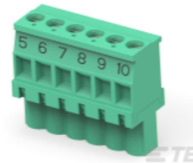
TE Part # 3-284041-2 TRMNL BLOK VT PLUG ST 6 POS SPL PRINT
