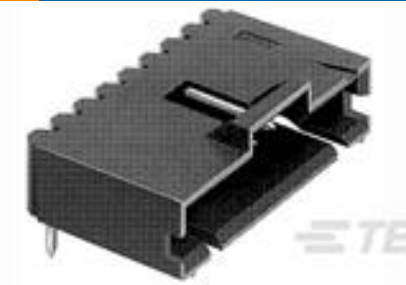
TE Part # 5-103635-4 05 MTE HDR SRRA LTCH.100CL LF
