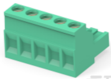
TE Part # 796634-5 5 POS 5.08MM R/A PLUG, TRM BLK
