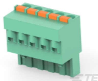
TE Part # 1986262-5 Female Spring Connector, Green, 5.08, 10
