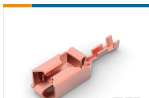
TE Part #928909-1 POSI LOCK RECP PLAIN
