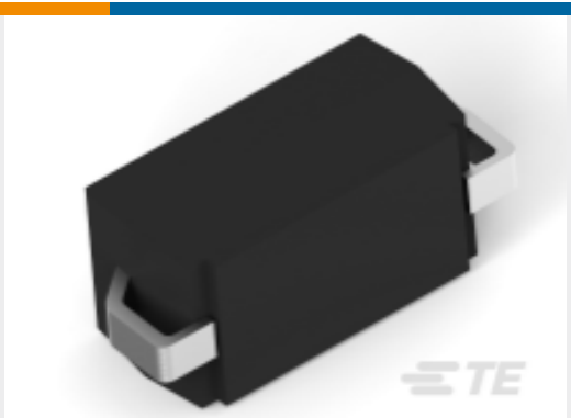
TE Part #1-2176324-7 SMV 3W 2M2 5%
