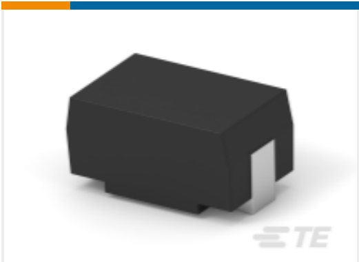
TE Part #6-1879234-6 SMD Power Resistor: 7 Watt, 200-2M Ohm
