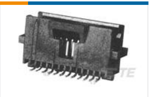
TE Part #5-104549-6 40 SYS50 S/M HDR DRST SHRDSN
