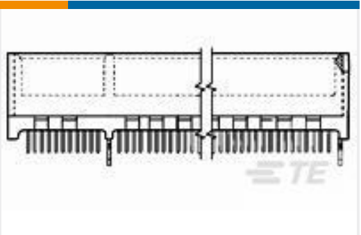
TE Part #5145167-4 STANDARD EDGE .050 SERIES 60 DUAL ASSY
