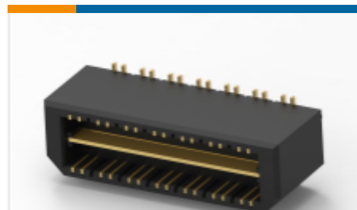
TE Part # 7-1658014-1 MSB0.80PL8ASY28DP,GP,10,VCTR
