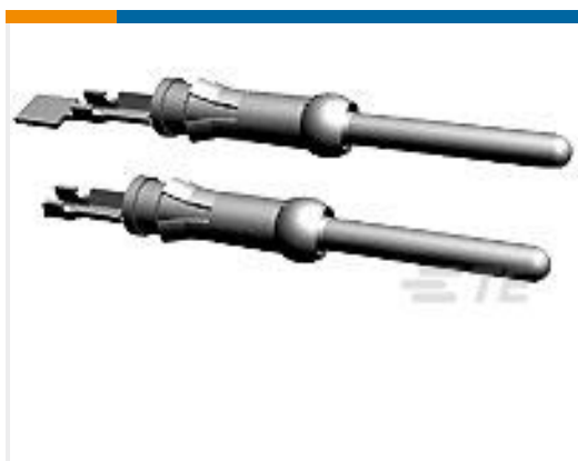
TE Part #66103-4 III+ PIN, 24-20, 30AU/FL, LP
