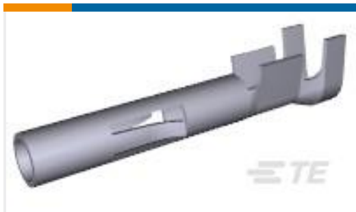
TE Part #350550-1 UMNL SOK 20-14 PTPBR L/P
