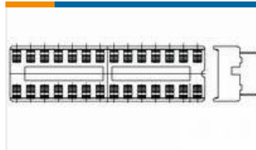
TE Part #1-2199298-6 20P,DIP SKT,300 CL,LDR,PB FREE
