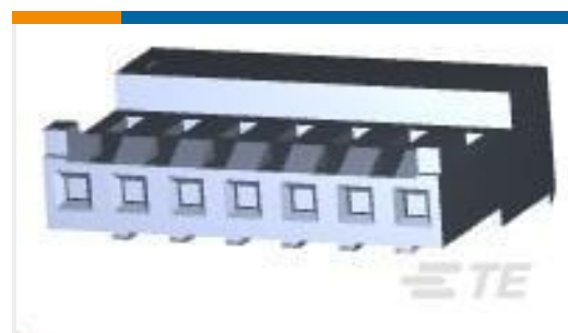
TE Part #3-644460-7 07P MTA156 CONN ASSY 18AWG ORA
