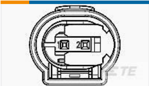
TE Part #284703-1 2POS MQS REC SEALED COD A
