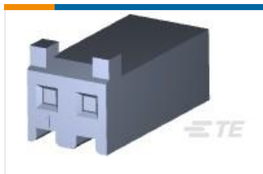
TE Part #770849-2 02P SL156 HSG W/LCK RMP & TABS
