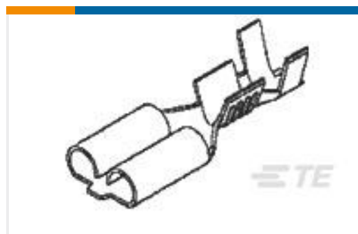
TE Part #170032-2 250 FASTON,REC.,20-14 AWG,BR
