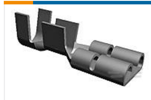
TE Part #63475-2 187 FASTON REC 20-16 AWG TPBR
