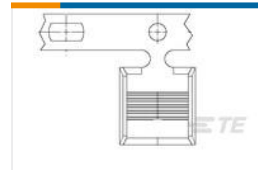
TE Part #1217990-2 AMVAR SPLC 6000-14000 025TPBR
