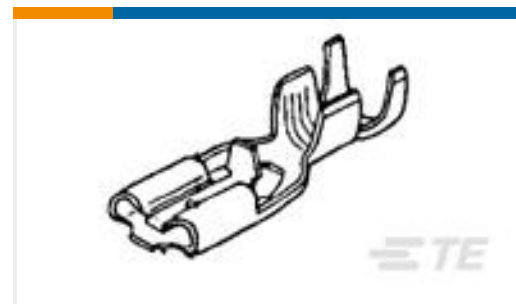
TE Part #170330-2 PL 187 RECEPTACLE 24-20 AWG NPPHBZ
